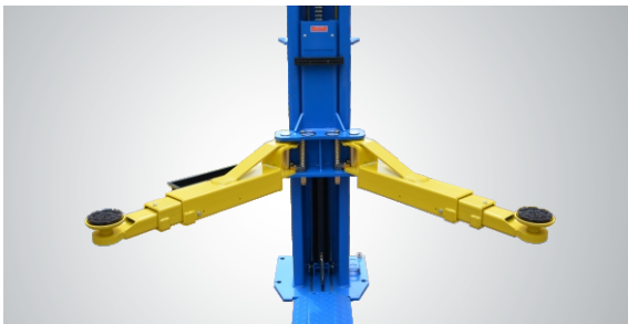
4 three-stages arms are suitable for more vehicles. Extremely high carriages, automatic arms restraints, protect rubber door guards, self-lubricated sliders... make PEAK compact line of two post lifts with many advanced features and high quality.
