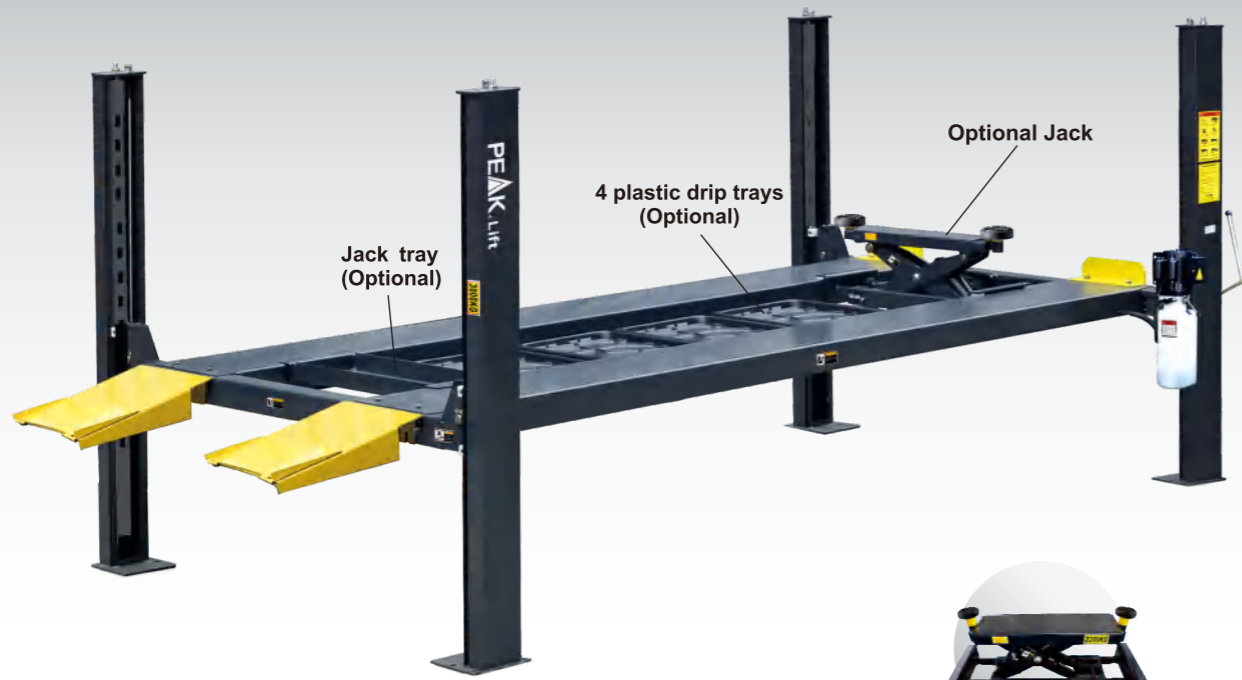
Optional J5H sliding jack with hand pump, 2.5" extension adapters included.
